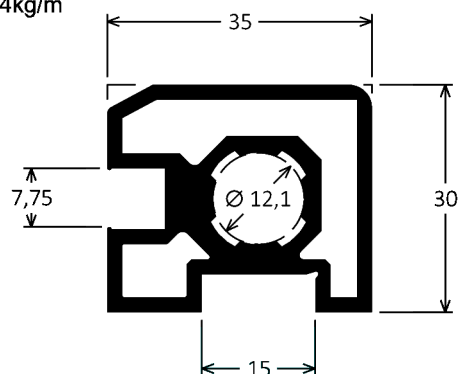
BK-357 1,144kg/m
