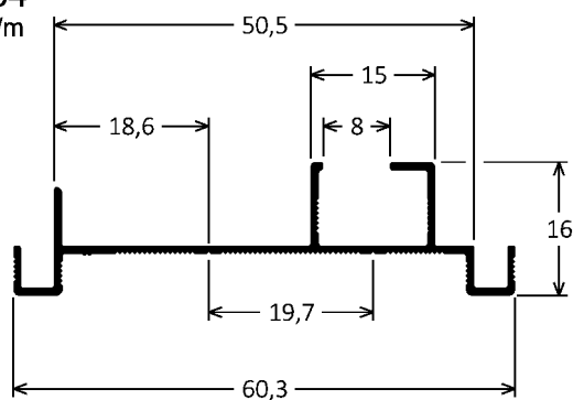
ISA-003 0,322kg/m
