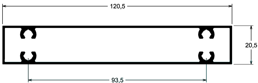
CX-947 1,193kg/m
