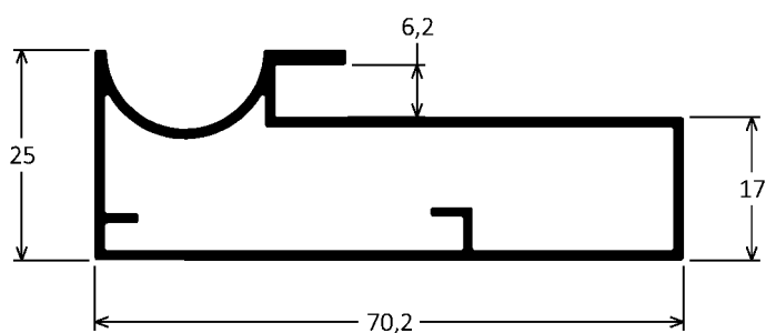
MV-034 0,708kg/m
