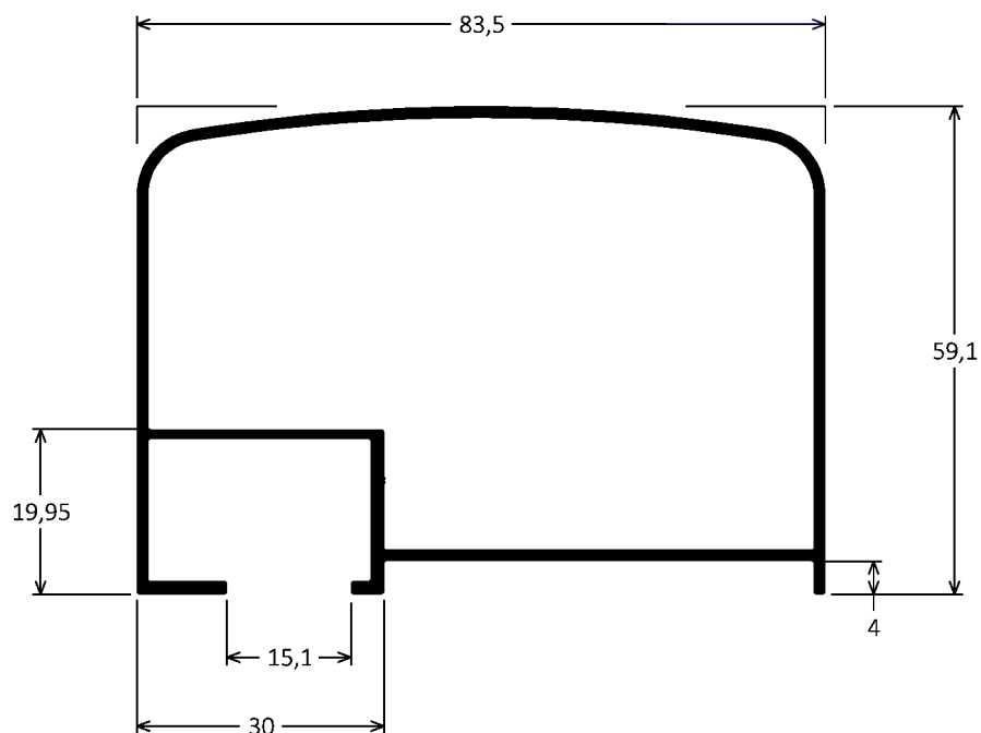
BX-115 1,135kg/m
